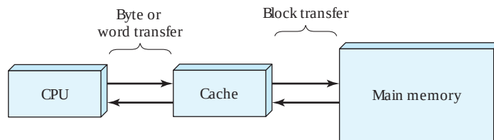
Figure 1.16 Cache and Main Memory
