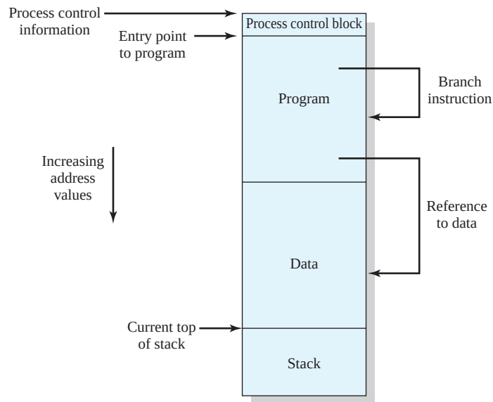
Figure 7.1 Addressing Requirments for a Process
