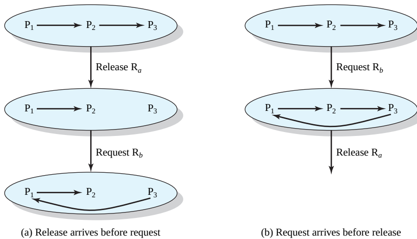
Figure 18.12 Phantom Deadlock
