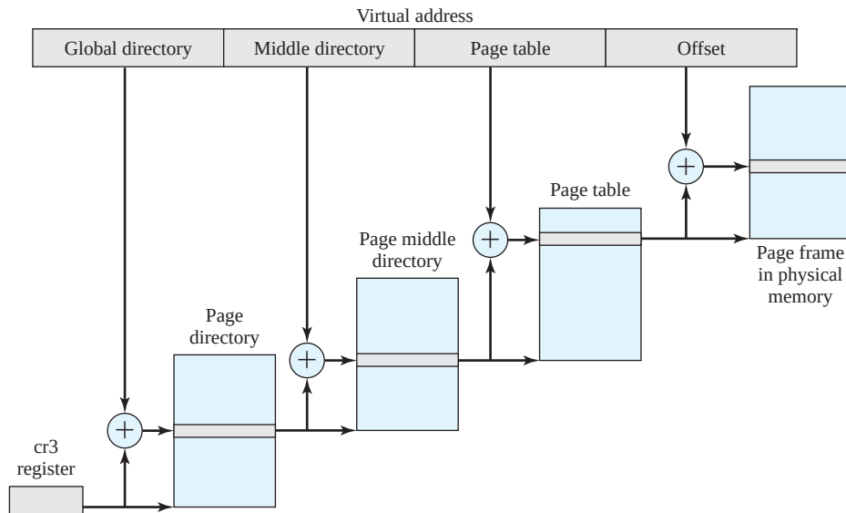
Figure 8.25 Address Translation in Linux Virtual Memory Scheme
